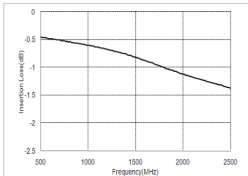
BW21S7511D01TF Insertion Loss Characteristics
