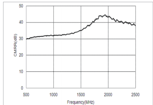
CMRR Characteristics
