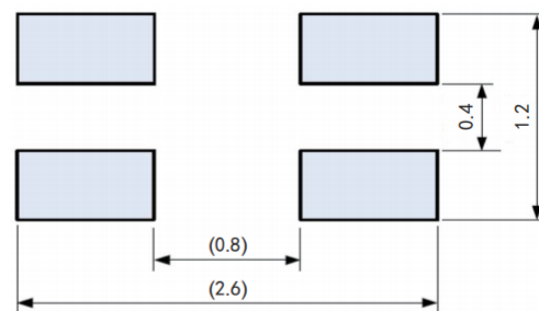
Land Pattern
