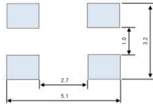
Land Pattern
