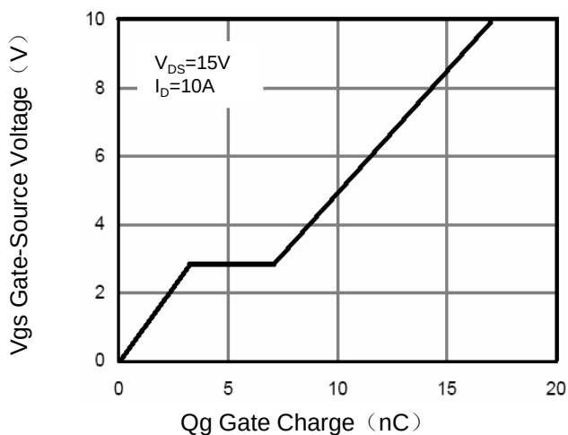
Figure 3. Gate Charge
