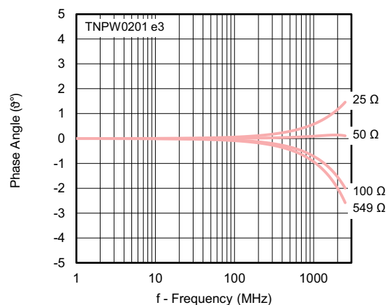
HF Performance (1)
