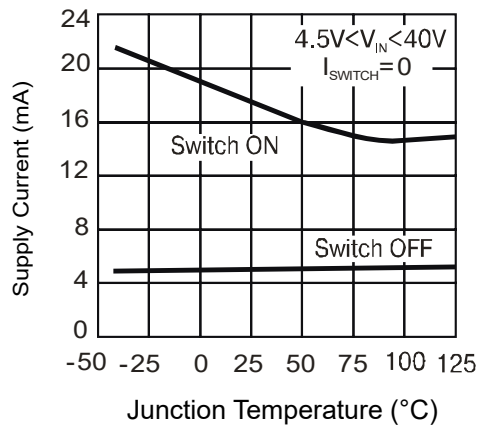
Figure 7: Operating Quiescent Current
