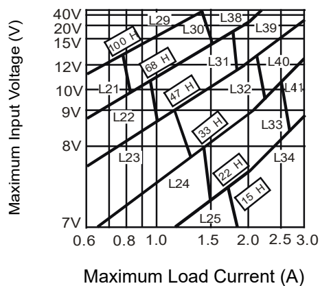
Figure 6: AP1501-5.0
