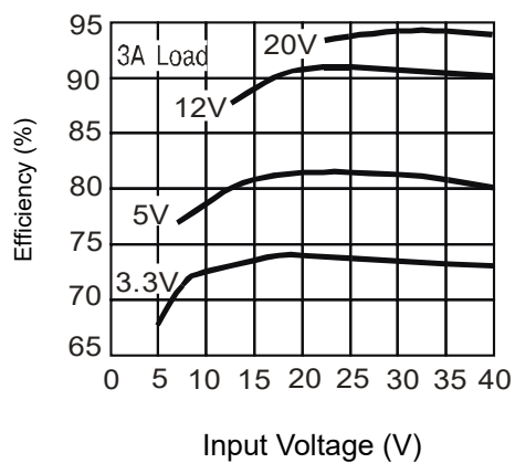
Figure 3: Efficiency
