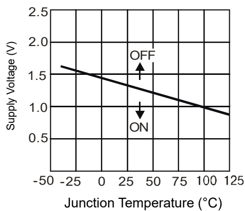
Figure 9: Minimum Operating Supply Voltage
