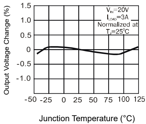
Figure 1: Normalized Output Voltage
