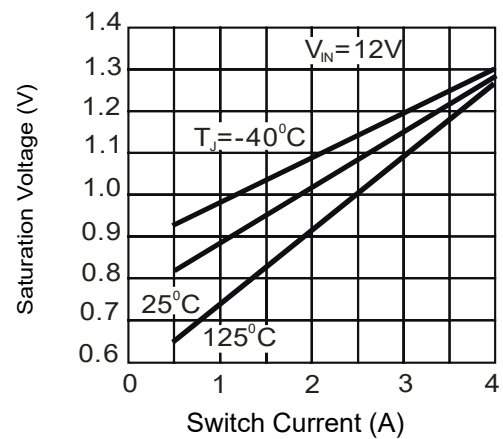
Figure 4: Switch Saturation Voltage
