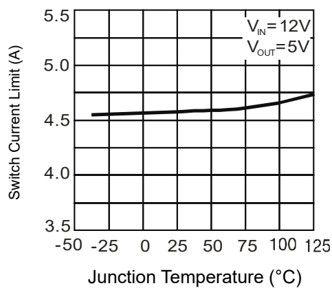
Figure 5: Switch Current Limit
