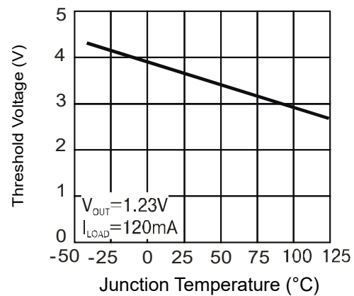
Figure 10: ON/OFF Threshold Voltage
