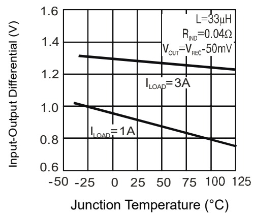
Figure 6: Dropout Voltage
