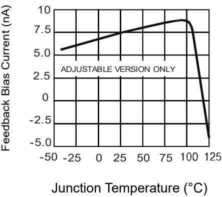
Figure 13: Feedback Pin Bias Current
