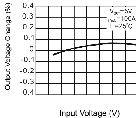
Figure 2: Line Regulation
