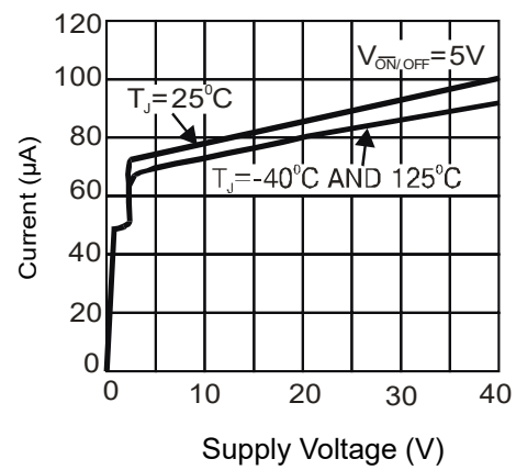
Figure 8: Shutdown Quiescent Current
