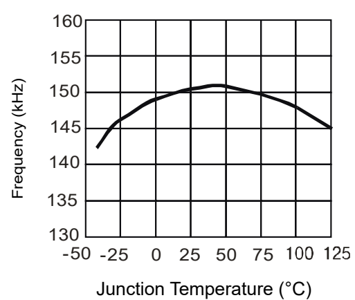
Figure 12: Switching Frequency
