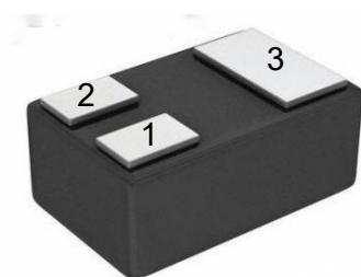
Package: DFN1006-3L 1: Base 2: Emitter 3: Collector
