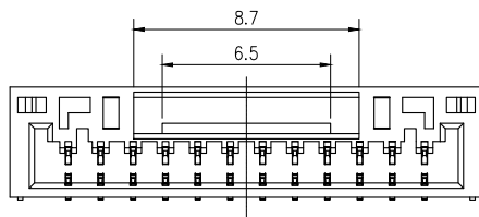
12PIN~13PIN
